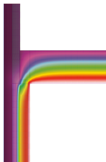
100mm partial fill insulation below gable detail
