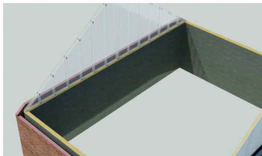
Trussed rafters not shown to aid illustration
