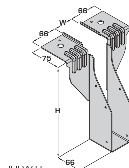
JHI-W-H Example: JHI-50-225
