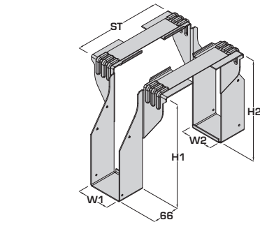
JHIST-W-H-ST or JHIST-W1-H1-ST-W2-H2 Example: JHIST-50-225-100 Example: JHIST-50-225-100-75-225
