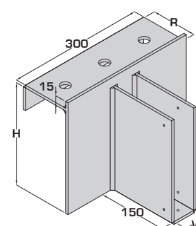
MASONRY-RTN-THICKNESS-W-H-R
