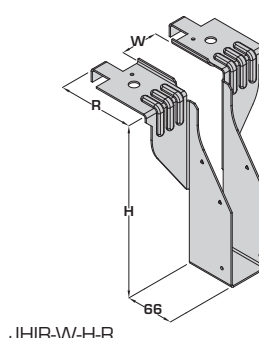
JHIR-W-H-R Example: JHIR-50-225-100 Only sizes marked (1) available (Returns available to suit 100mm block work only)
