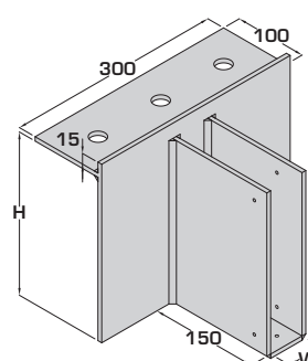
MASONRY-STD-THICKNESS-W-H
