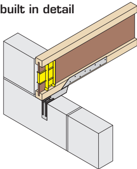
PST strap with non-restraint hanger
