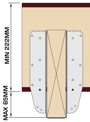
UH OR HUH* – 220MM DEEP
