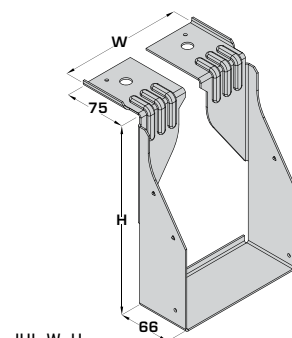
JHI-W-H Example: JHI-150-225
