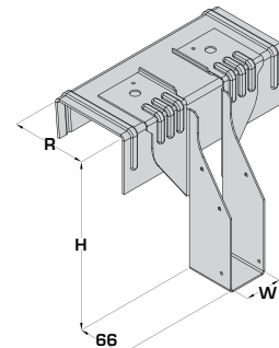
RB-JHIR-W-H-R Example: RB-JHIR-50-225-100 Only sizes marked (1) available (Returns available to suit 100mm block work only)
