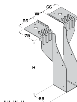
JHI-W-H Example: JHI-50-225
