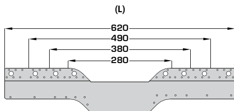
MHE/MHI FLAT BLANK (280 – 620)
