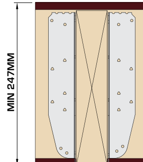
UH OR HUH* – 235MM DEEP (235–254mm deep joists)
