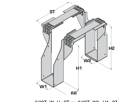
JHIST-W-H-ST or JHIST-W1-H1-ST-W2-H2 Example: JHIST-50-225-100 Example: JHIST-50-225-100-75-225
