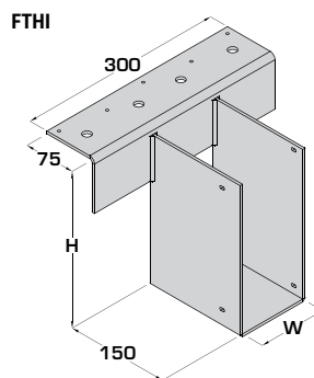
FTHI-W-H Example: FTHI-100-245
