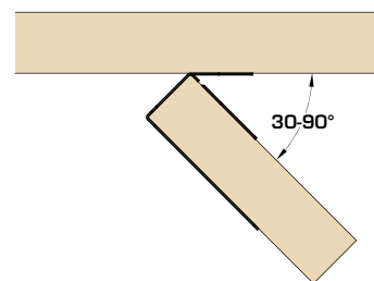
Left hand skew (skews between 30-90^{\circ} )
