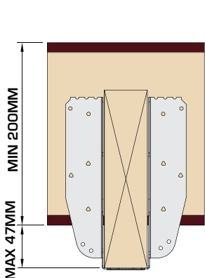
UH OR HUH* – 195MM DEEP
