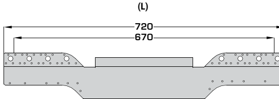
MHE/MHI FLAT BLANK (670 - 720)
