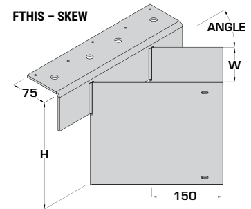
FTHIS-W-H-OFFSET DIRECTIONAL-ANGLE Example: FTHIS-100-245-L-45 (skews from 30°-87.5° in 2.5° increments, with 5mm automatically added to ordered width to allow for tolerance)
