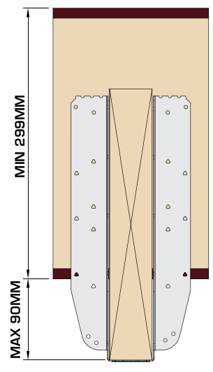
UH OR HUH* – 300MM DEEP
