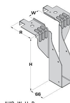
JHIR-W-H-R Example: JHIR-50-225-100
