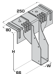
RB-JHI-W-H Example: RB-JHI-50-225
