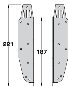
UH-195 (To suit 195 – 200mm deep i-joists)
