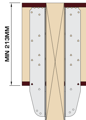
UH OR HUH* – 300MM DEEP (300–304mm deep joists)
