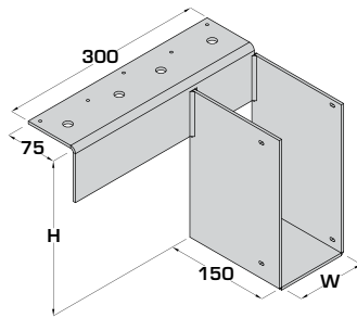
FTHIO-W-H-OFFSET DIRECTION Example: FTHIO-100-245-L FTHIO-100-245-R
