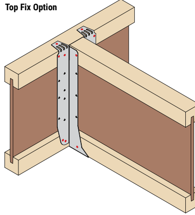
Top Fix Option
